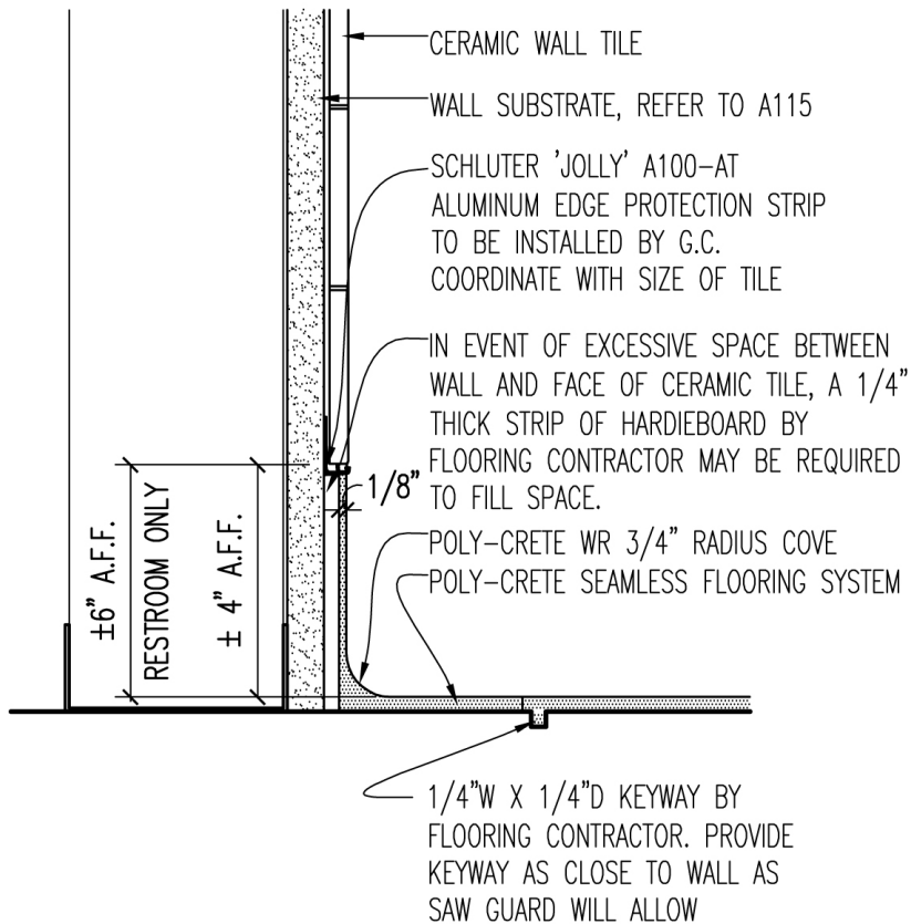
9A POLYCRETE BASE DETAIL @ TILE TO POLYCRETE A125 3" = 1'-0"
